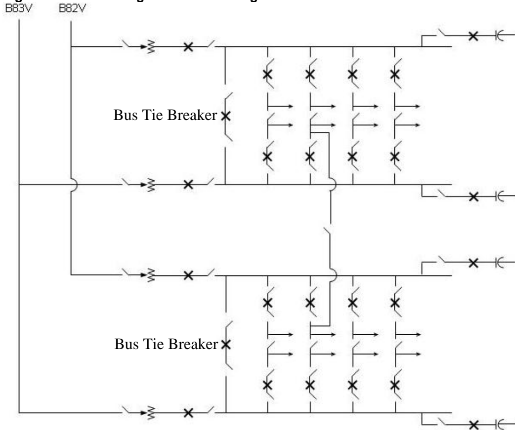
Figure 1: DESN Configuration at Armitage TS
