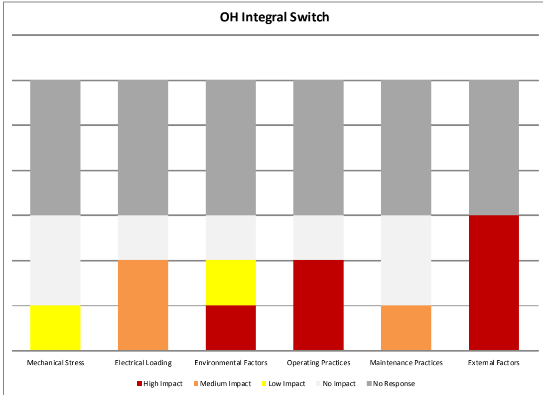
Figure 7-2 Impact of Utilization Factors on the Useful Life of Overhead Integra Switch
