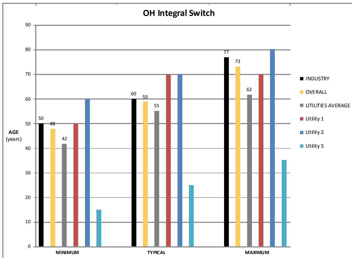
Figure 7-1 Useful Life Values for Overhead Integra Switch
